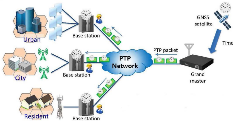
Figure 7: PTP network configuration.
