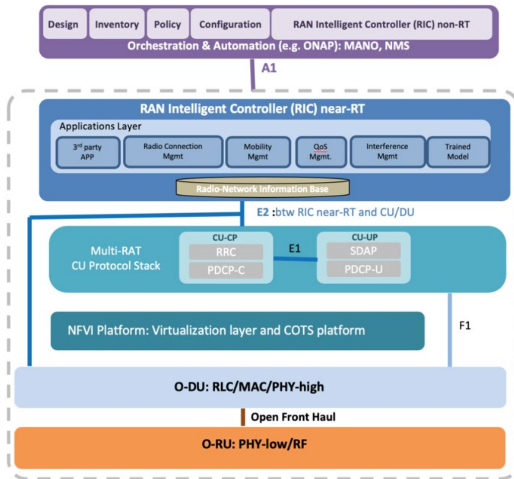
Figure 4: O-RAN open system architecture
