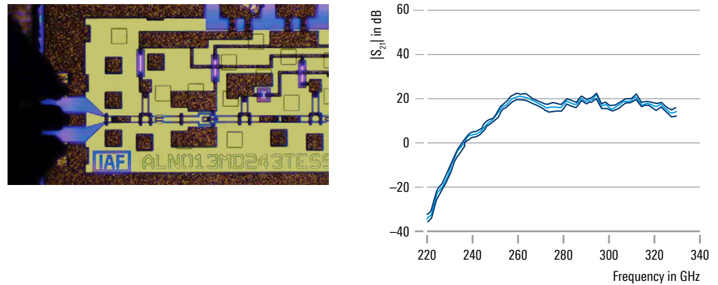
Figure 12: Fraunhofer IAF four-stage, 325 GHz MMIC LNA (left) and measured scalar gain |S_{21}| with the \pm 95\% confidence intervals (right) [35]
