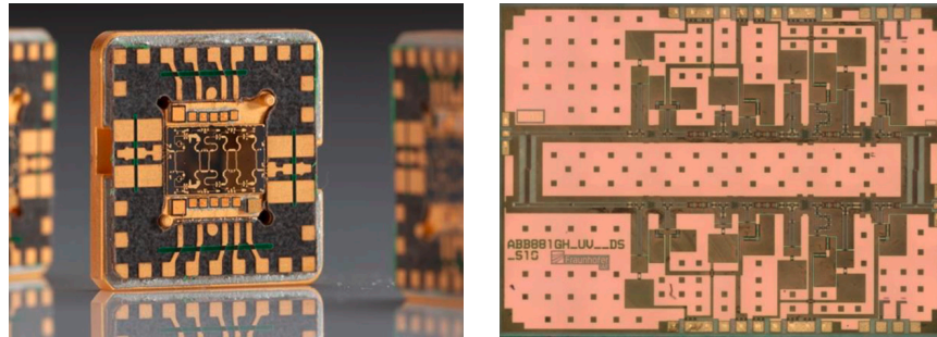
Figure 14: 27 GHz to 41 GHz GaN/SiC MMIC amplifier in proprietary SMT compatible package (left); 40 GHz to 70 GHz GaN/SiC MMIC amplifier (right)
