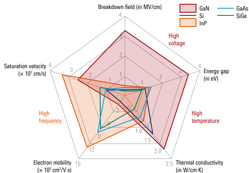
Figure 24: Comparison of selected material properties of mmWave semiconductors [62]
