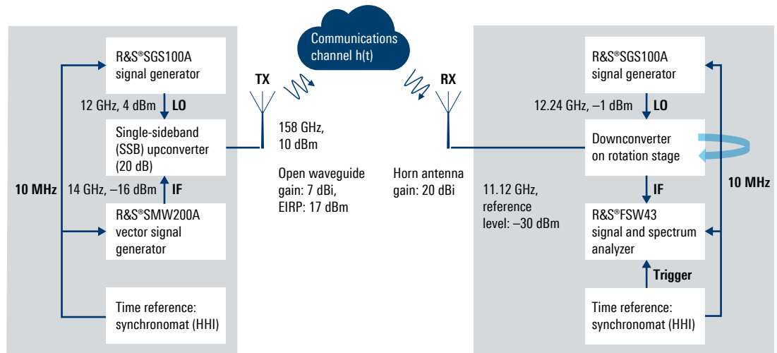
Figure 29: Block diagram of the channel sounding measurement setup for 158 GHz
