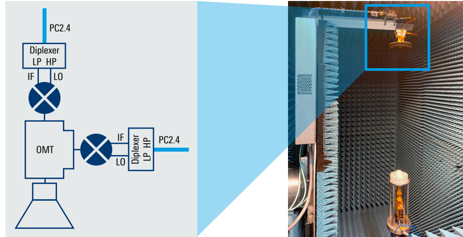
Figure 17: Measurement setup using a compact spherical scanning system with frequency converted probe and DUT at the azimuth pole
