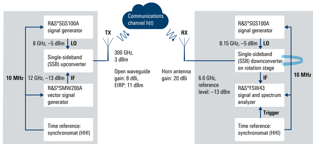
Figure 27: Block diagram of the 300 GHz channel sounding system
