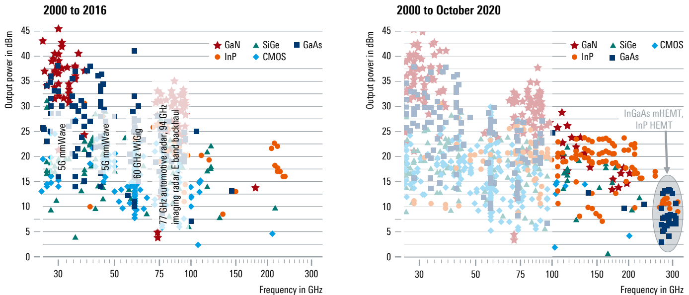
Figure 25: Overview of state-of-the-art high frequency power amplifiers as of September 2016 (left) and October 2020 (right) [64] [65]
